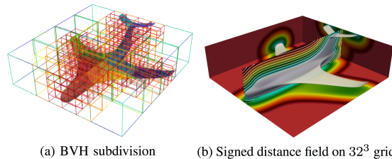
Fig. 1. Signed distance of generic jet configuration ( \sim 375K surface elements).
