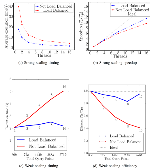
Fig. 3. Preliminary performance results: Strong and weak scaling.
