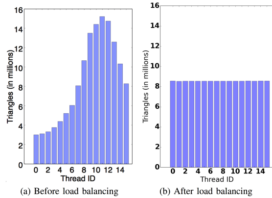
Fig. 2. Number of point-triangle intersection tests per thread on a 16 thread run before (a) and after (b) load-balancing with RAJA IndexSets
